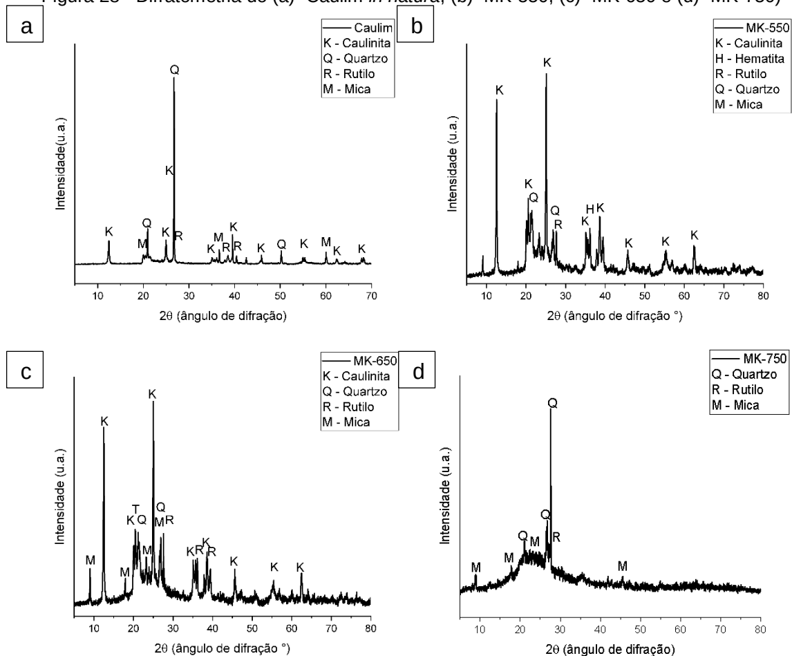
Figura 28 - Difratometria do (a)- Caulim in natura , (b) -MK-550, (c) -MK-650 e (d) -MK-750
